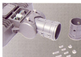
Double casting installation design
