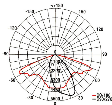
Vertical tilt adjustment 0 deg - 10 deg
